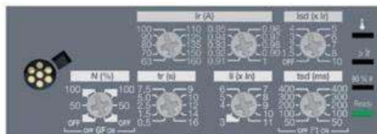
Trip unit LSI
